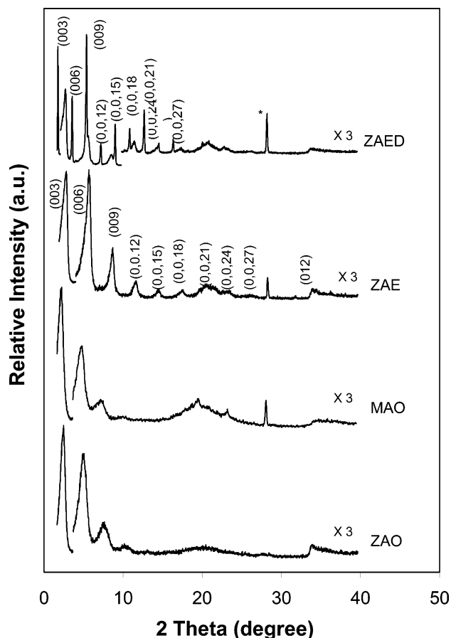
Figure 2. XRD patterns of samples ZAO, ZAE, ZAED, and MAO. The peak marked with an asterisk (*) is from internal calibrant \text{CaF}_2 . The peak between (003) and (006) for ZAED is attributed to ZAE impurity.
