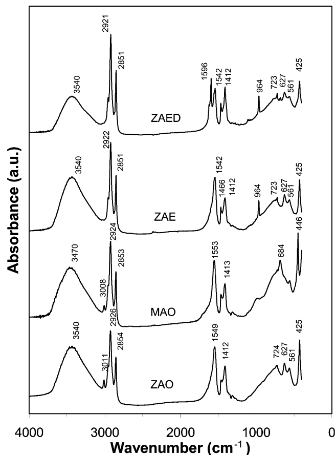
Figure 1. FTIR spectra of samples ZAO, ZAE, ZAED, and MAO.
