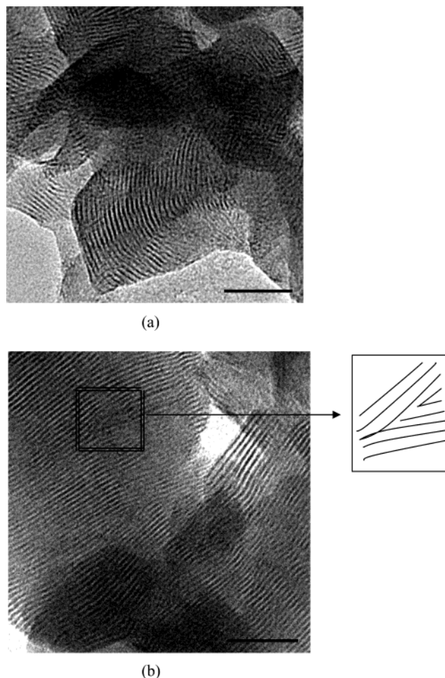
Figure 5. Transmission electron micrographs of (a) ZAO and (b) ZAE; scale bar 50 nm.
