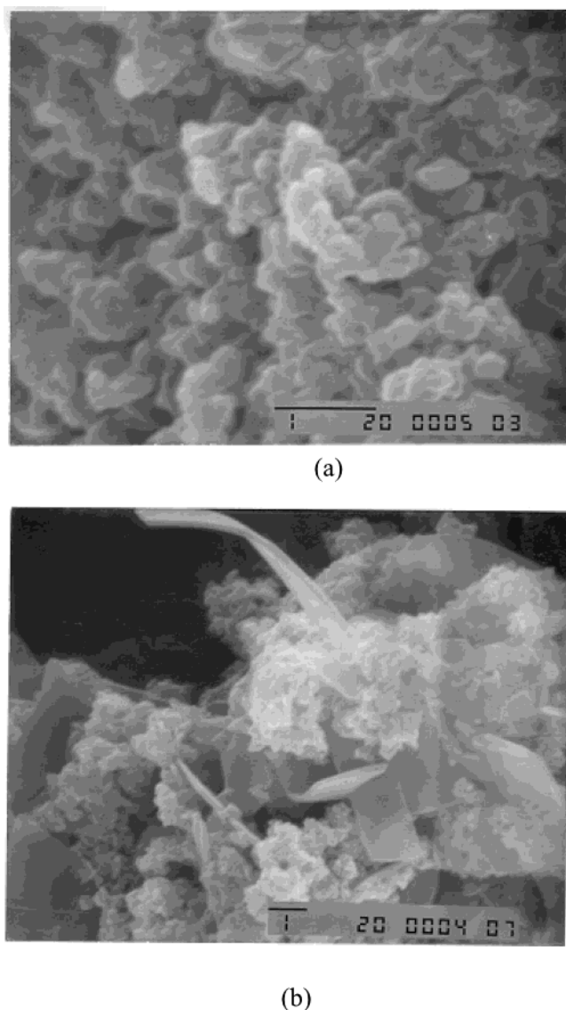
Figure 4. Scanning electron micrographs of (a) ZAO and (b) ZAE; scale bar 1 \mu\text{m} .
